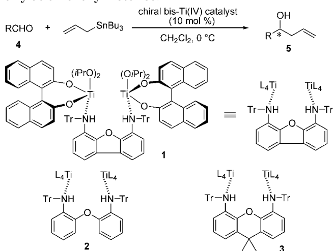
Scheme 1. Catalytic asymmetric allylation of aldehyde 4 with allyltributyltin in the presence of the chiral bis-Ti(IV) complexes 1–3 [ L_4 = ((S)\text{-binaphthoxy})(\text{OiPr})_2 ]
